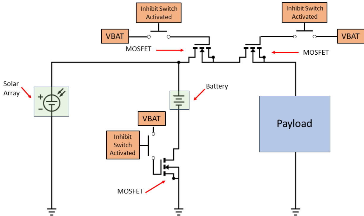
Figure 4.2.1-1: CubeSat Electrical Subsystem Block Diagram (Note: RBF pins not shown)
