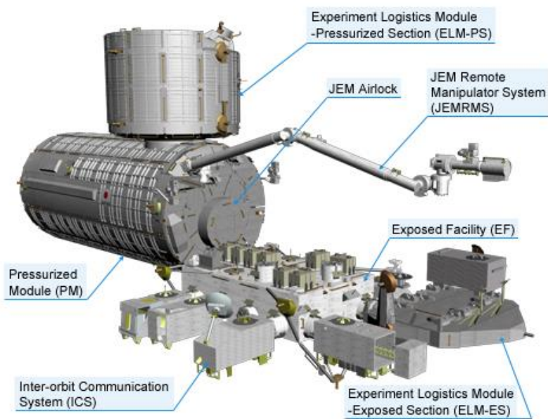
Figure 3.4.3.4-2: JEM Overview
