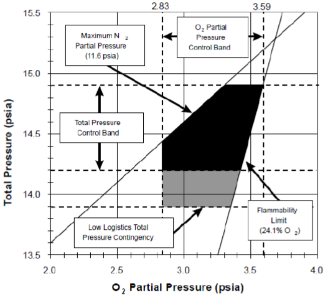
Figure 3.4.3.2-2: Operating Limits of the ISS Atmospheric Total Pressure, and Nitrogen and Oxygen Partial Pressures (Ref SSP 57121)
